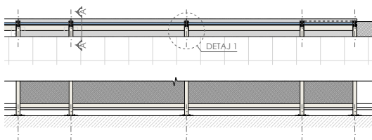
DETAJ 1 Sh. 1:10
